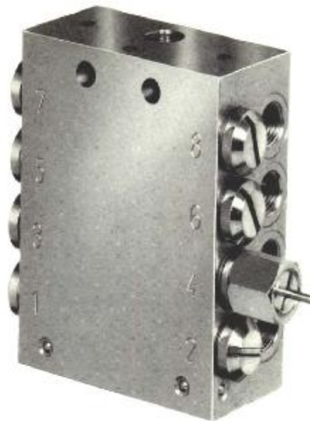
Quicklub Metering Device
